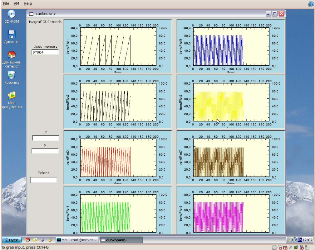
Fig. 3 Examples of HMI from ISaGRAF target system
